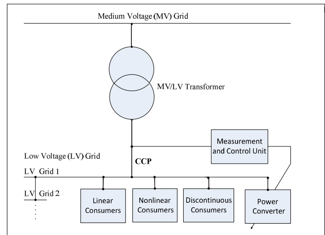
Fig.2. Power grid diagram with harmonics compensation based on PWM controlled power electronic converters
