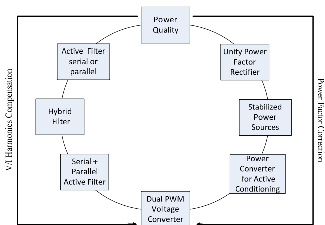
Fig.1. Unitary diagram of power electronic converters used in distortion and power factor compensation of MV/LV grids.
